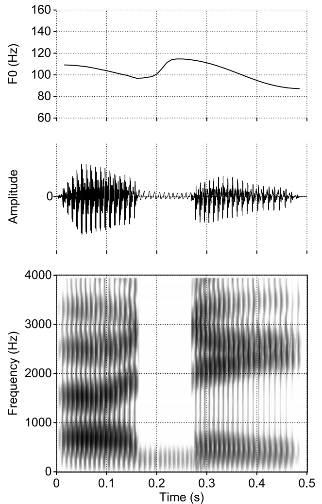
Figure 6. Example of the fundamental frequency (F0) contour, waveform, and spectrogram of a synthetic speech sample produced in the [əCi] environment with l_c = 14.3 cm. The top panel shows the F0 contour, the middle panel is the speech signal, and the bottom panel is the wide-band spectrogram of the speech signal. Waveforms such as this were converted to audio files for presentation in the listening experiment.
