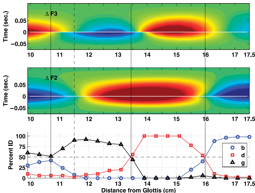
Figure 7. Contour plots based on the formant deflections determined with Equation 3 for all 20 time-varying area functions in the [əCi] set and associated identification (ID) functions from the listening experiment. The middle and upper panels correspond to \Delta F2 and \Delta F3 , respectively. The x -axis of each plot represents the portion of the vocal tract length within which constrictions were imposed to generate the set of VCVs. The y -axis in the middle and upper plots is time, where 0 s represents the point of vocal tract closure and release. Negative and positive time correspond to the constriction onset and offset periods, respectively. Like colors within each plot are contours where the formant deflections are constant. The solid vertical lines indicate phonetic boundaries defined by the 50% crossover points on the ID curves. The dashed lines are alternative boundaries discussed in the text.
