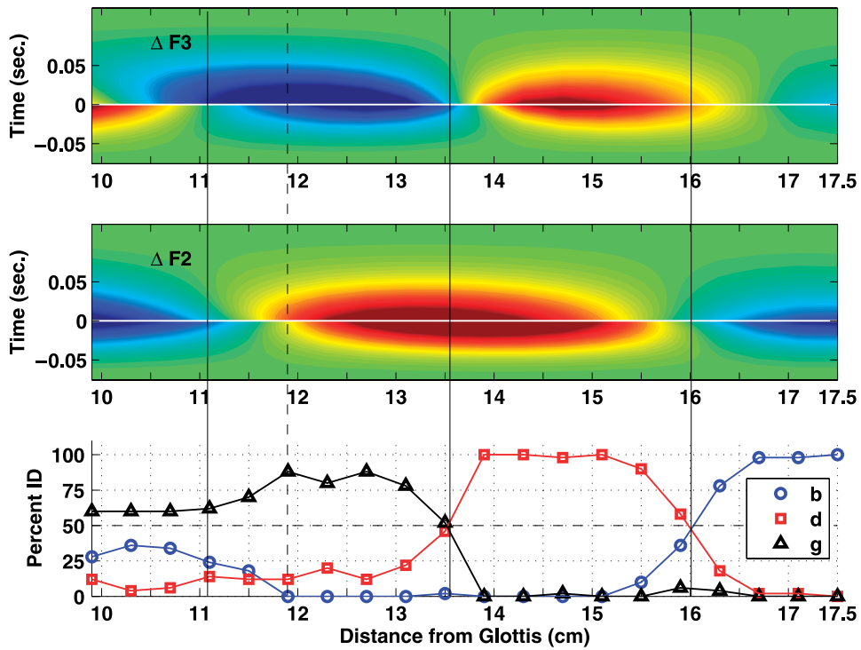
Figure 8. Contour plots based on the formant deflections determined with Equation 3 for all 20 time-varying area functions in the [əCa] set and associated ID functions from the listening experiment.
