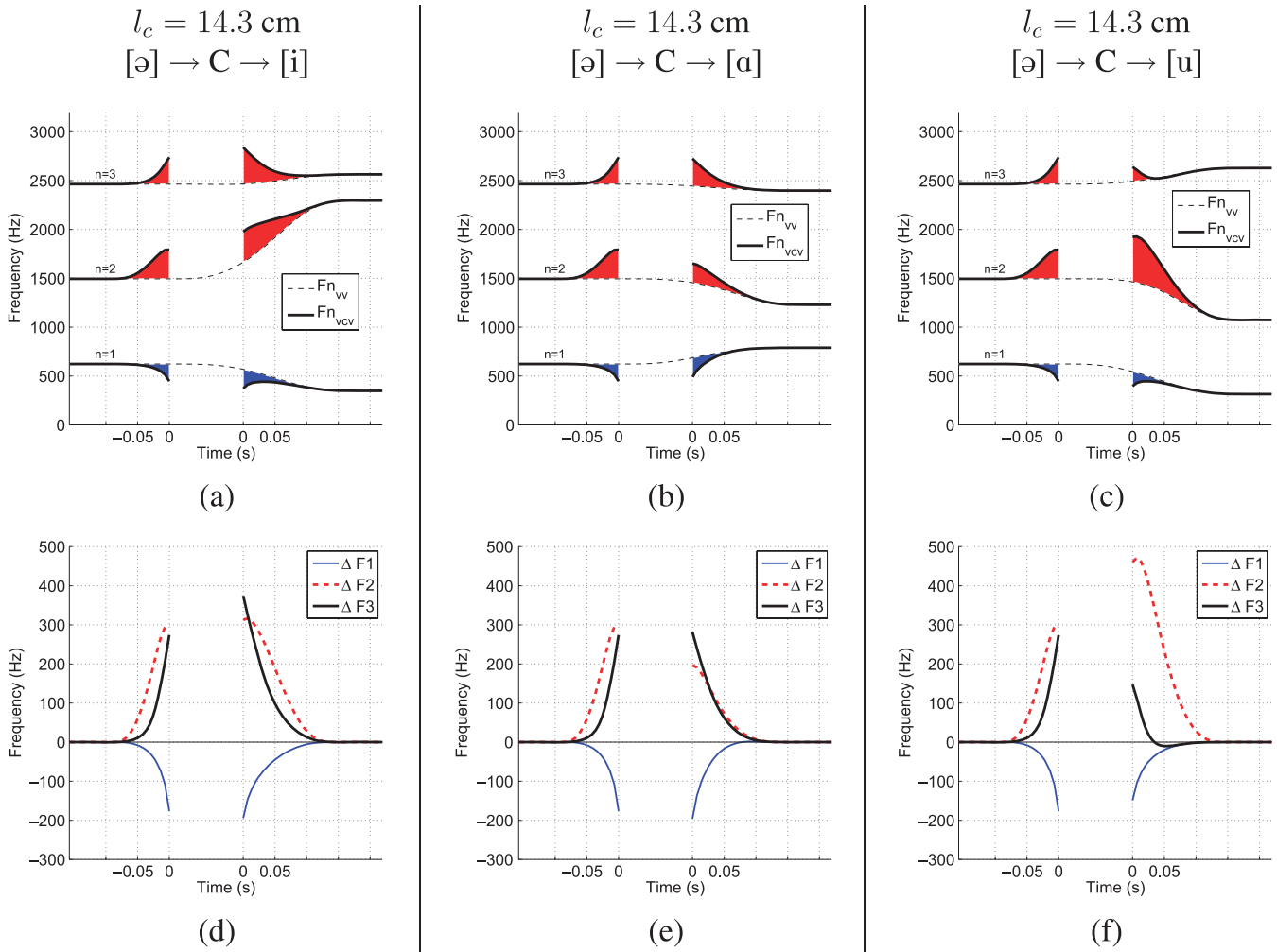
Figure 4. Formant frequencies and formant deflections calculated for time-varying area functions of vowel-to-vowel (VV) transitions and VCVs, similar to those in Figures 3a and 3c. For the plots in the top row (a, b, c), dashed lines indicate the calculated formants for each VV transition only, whereas the thick solid lines are the formants for the VCV. The shaded portions indicate the deflection of the formant frequencies generated by the VCV away from those generated by the VV alone (red indicates an upward deflection, and blue indicates a downward deflection). The plots in the bottom row (d, e, f) show time-dependent differences (deflections) between the formant frequencies generated by the VCV relative to those generated by the VV alone, on the basis of Equation 3. Negative and positive times on the x-axis of each plot denote the constriction onset and offset periods, respectively. The time between the two “zero” points is the period of vocal tract occlusion. Each column of plots corresponds to a VV context of [əi], [əa], or [əu], and the constriction location is l_c = 14.3 cm for all three cases.
