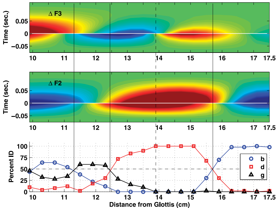
Figure 9. Contour plots based on the formant deflections determined with Equation 3 for all 20 time-varying area functions in the [əCu] set and associated ID functions from the listening experiment.
