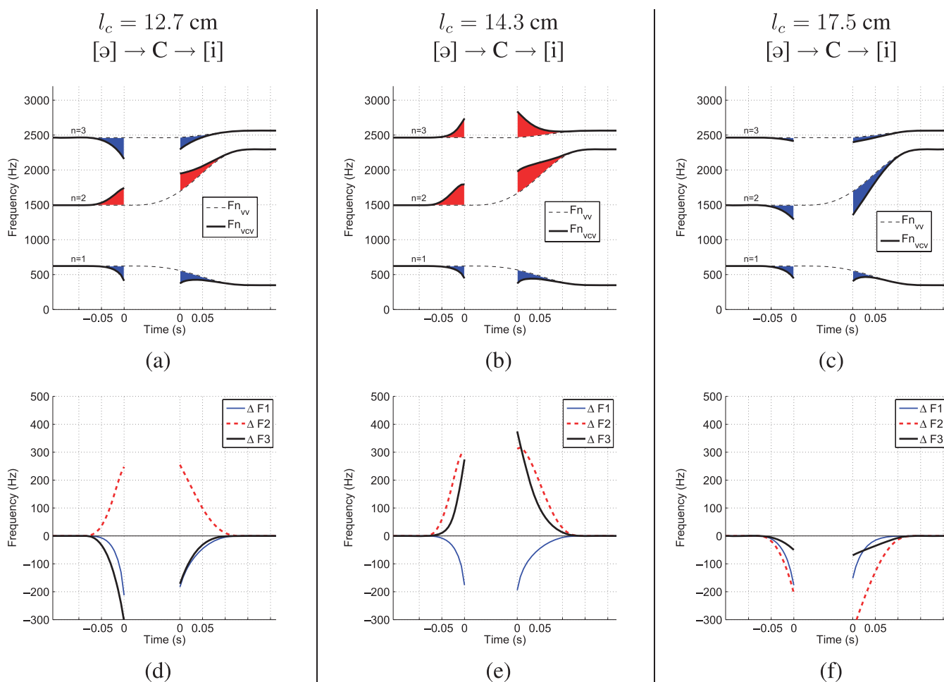
Figure 5. This figure has the same layout as that of Figure 4, but the difference is that the vowel context was kept constant as [əi], and the constriction location was set to 12.7 cm, 14.3 cm, and 17.5 cm, respectively, across the three cases.
